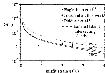
FIG. 4. The critical geometry G(T) of intersecting (lower curves) and isolated islands (upper curve) required for the nucleation of 60^\circ half loops. Relevant experimental data points are superimposed on the curves (see text).
