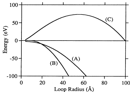
FIG. 3. Total energy curves for nucleation of a 60^\circ half loop in a \text{Si}_{0.5}\text{Ge}_{0.5} alloy as a function of loop radius R_L . The curves A and B correspond to the cusp functions C^A(R_L) and C^B(R_L) , and C is the flat surface solution corresponding to C^C(R_L) (see text). The cusp geometry ( d=7 nm, \rho_v=3 nm) is appropriate to Fig. 1. The calculation assumes \alpha=4 .
