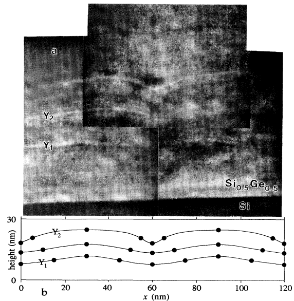
FIG. 1. (a) [110] Z-contrast image of a \text{Si}_{0.5}\text{Ge}_{0.5} alloy grown by MBE with 0.25 nm Ge marker layers deposited at selected intervals. The growth temperature was 400 °C and the deposition rate 2 \text{ \AA s}^{-1} . The profile simulations in (b) correspond to the period of cusp formation in (a) between vertical ordinates Y_1 and Y_2 . The solid circles denote the peak, valley, and inflection positions as determined from Eqs. (3), (4), and (5) (see text).
